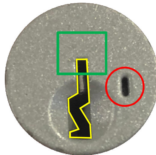
SC1 Keyway "C-Keyway"
